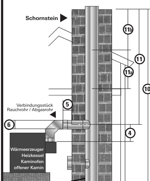
Schornstein
