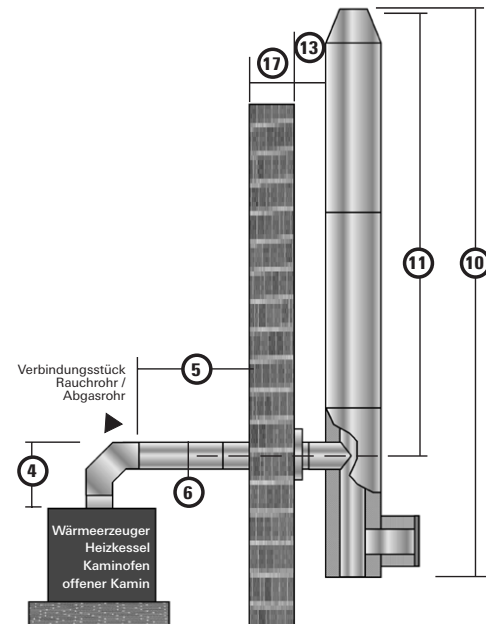
Kamin
